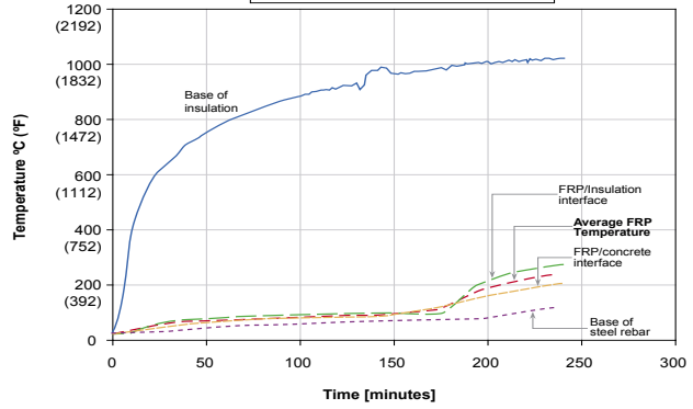
Fig. 1: Slab 2 Temperatures
